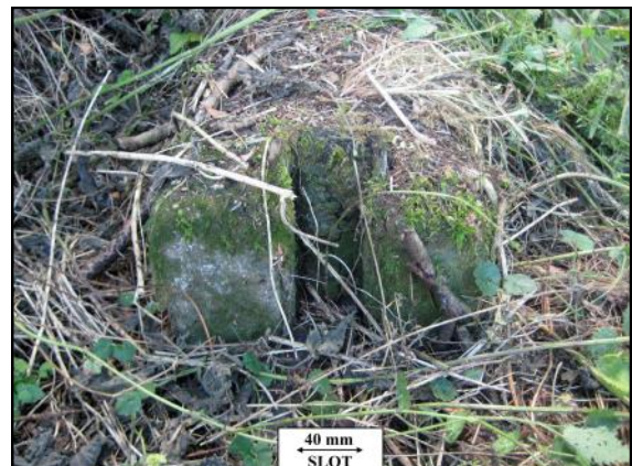
Figure 2: A close up showing the remains of one of the water channels and the slot for a control board. U-shaped iron channels were set into each slot to allow the boards to be adjusted easily. A few remain in situ. Most were probably removed for scrap many years ago.
